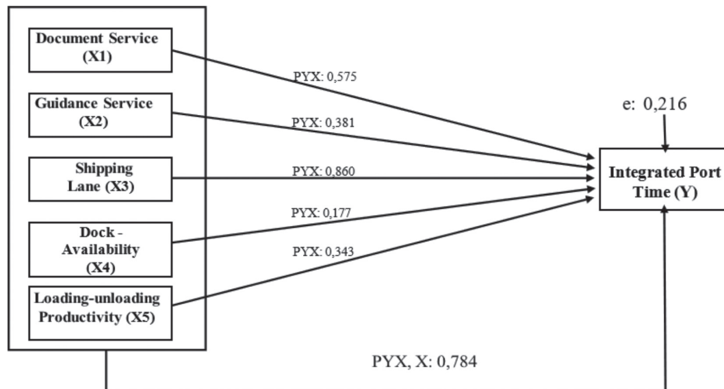
Figure 2 Path Analysis Diagram
